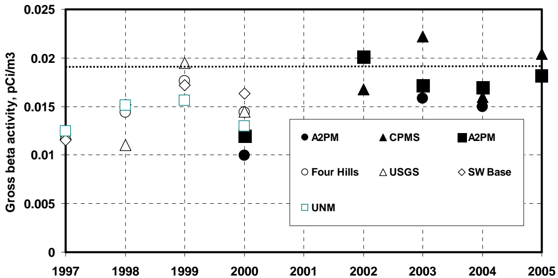
Figure 3-9 Comparison of reported data for gross beta activity in air at locations sampled by SNL (A2PM, CPMS, A2PM) with those sampled by NMED (Four Hills, USGS, SW Base, UNM); the 40CFR61 level for environmental compliance for Am-241 is indicated with a dotted line.
