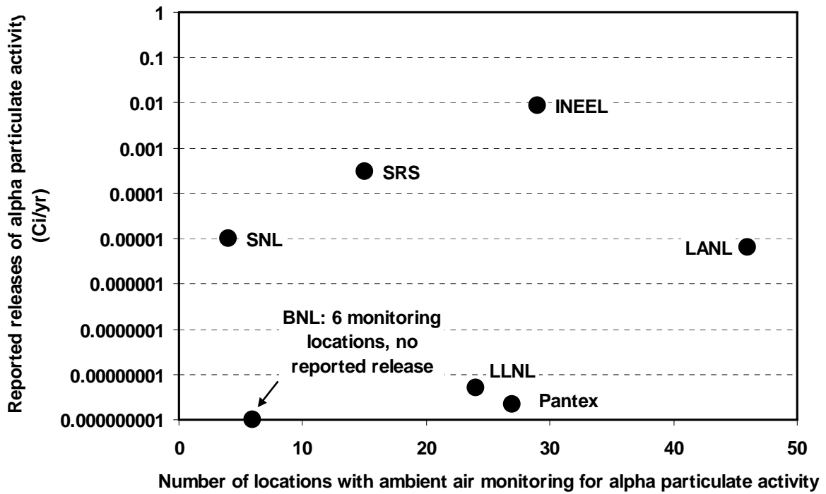
Figure 4-2 Number of locations at selected DOE facilities with ambient air monitoring for alpha particulate activity as a function of the reported releases of airborne alpha particulate activity
