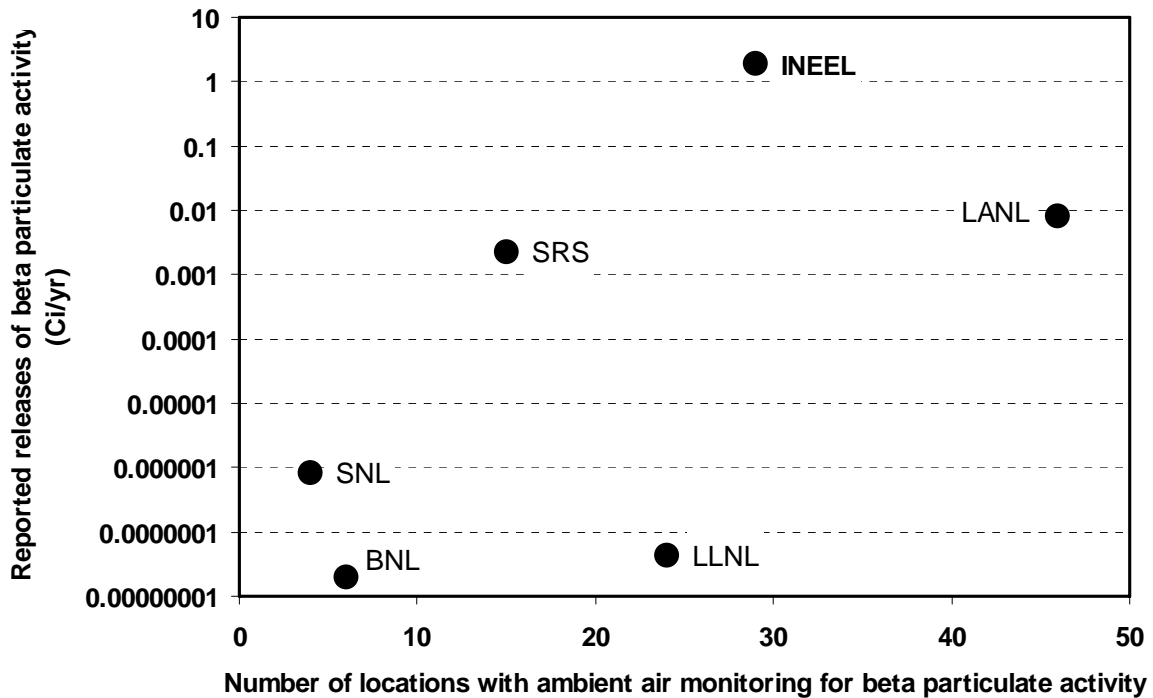
Figure 4-3 Number of locations at selected DOE facilities with ambient air monitoring for beta particulate activity as a function of the reported releases of airborne beta particulate activity
