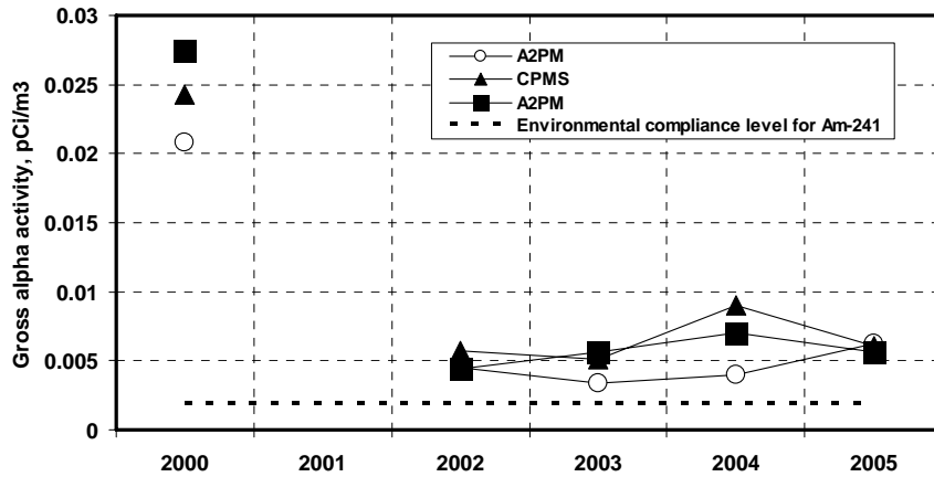
Figure 3-2 Reported levels of gross alpha activity at ambient air sampling locations at SNL, 2000 through 2005
