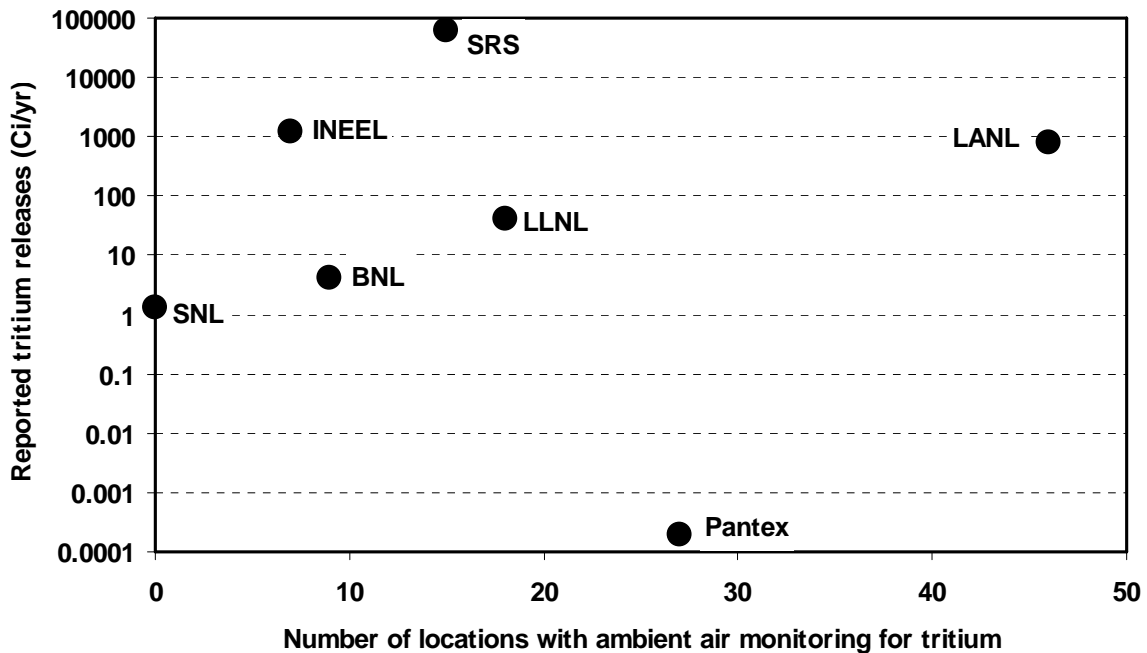
Figure 4-1 Number of locations at selected DOE facilities with ambient air monitoring for tritium as a function of the reported releases of airborne tritium
