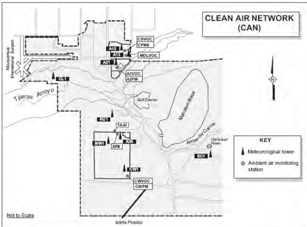
Figure 3-1 Sampling locations radionuclides in air at SNL as of 2005 (SNL, 2006a)
