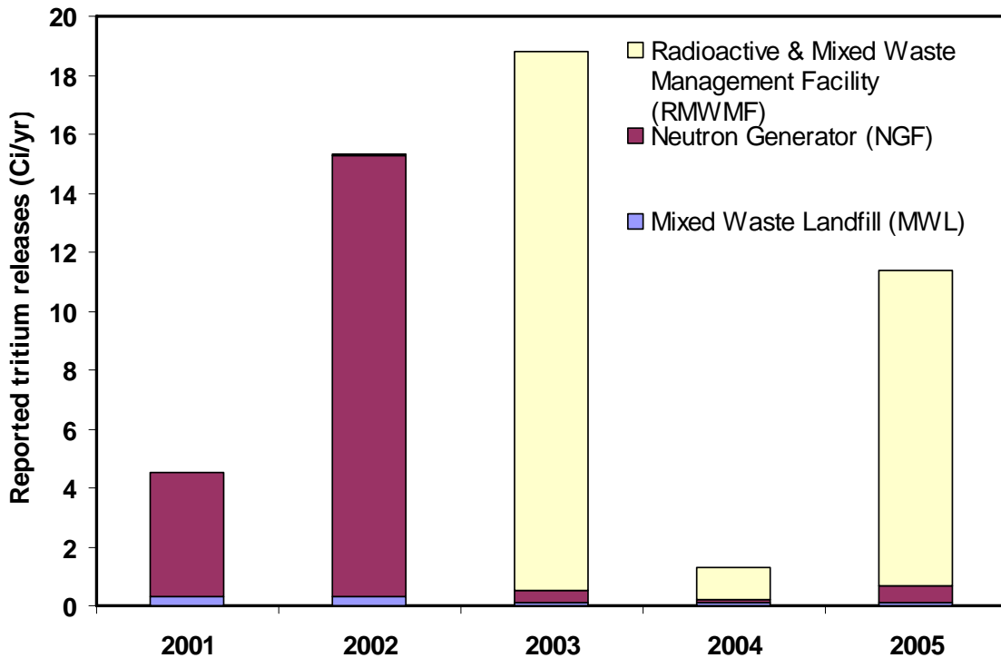
Figure 2-2 Reported releases of tritium from major sources at SNL, 2001 - 2005
