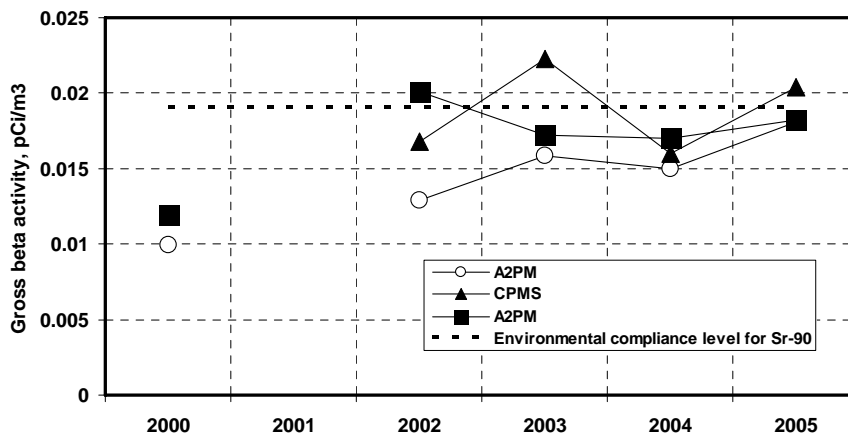
Figure 3-3 Reported levels of gross beta activity at ambient air sampling locations at SNL, 2000 through 2005
