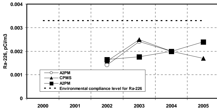
Figure 3-5 Reported levels of Ra-226 at ambient air sampling locations at SNL, 2000 through 2005
