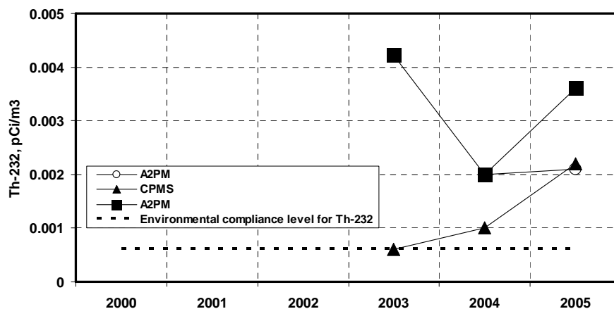
Figure 3-6 Reported levels of Th-232 at ambient air sampling locations at SNL, 2000 through 2005
